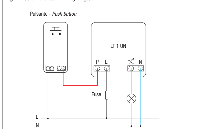
Fig. 1 - Schema base - Wiring diagram
