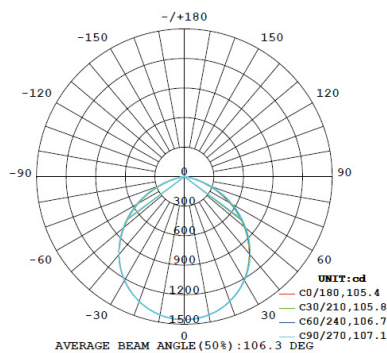
LIGHT DISTRIBUTION 62594
