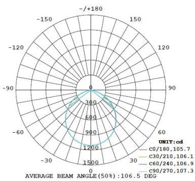
LIGHT DISTRIBUTION 62593
